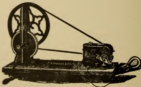
Fig. 39. DYNAMO—HAND-POWER, FOR ELECTRO-PLATING, ETC.
